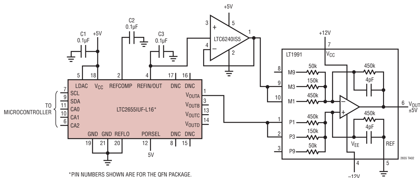
±5V Bipolar Output DAC
